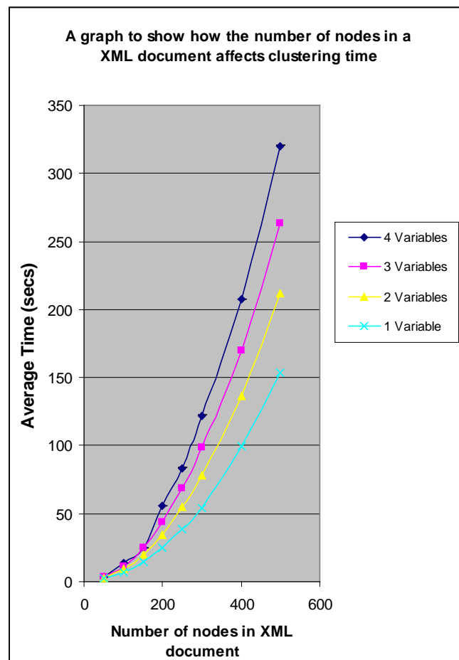
Graph 2 The number of nodes against time
