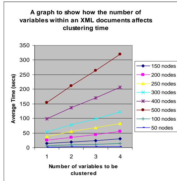
Graph 1.Number of variables against time
