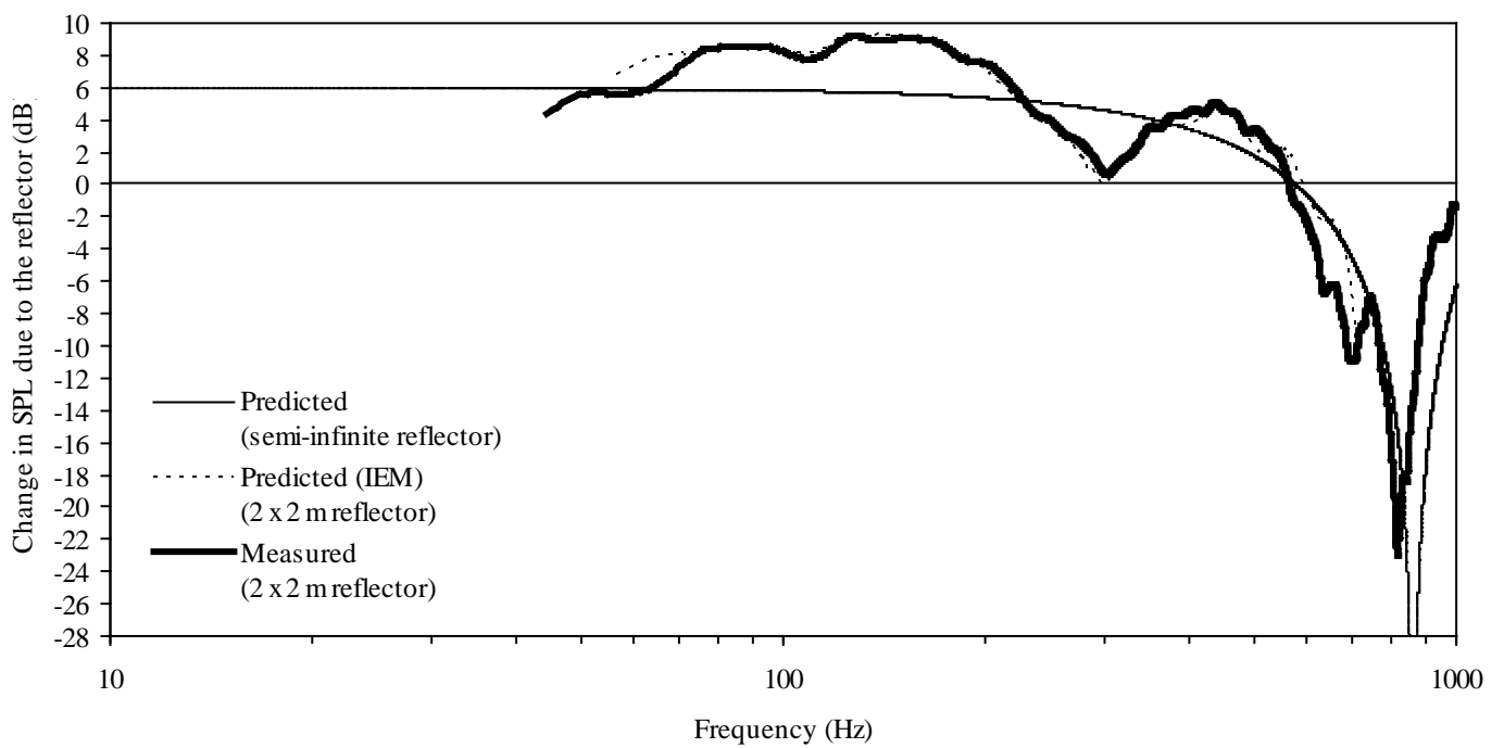
Fig. 5 Change in the sound pressure level due to the presence of the reflector: receiver-reflector distance, d=0.1 m.
