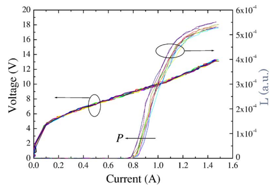
FIG. 3. (Color online) Pressure dependence of the measured L - I - V characteristics at 115 K taken in the range of P=0 to P=5.5 kbars.
