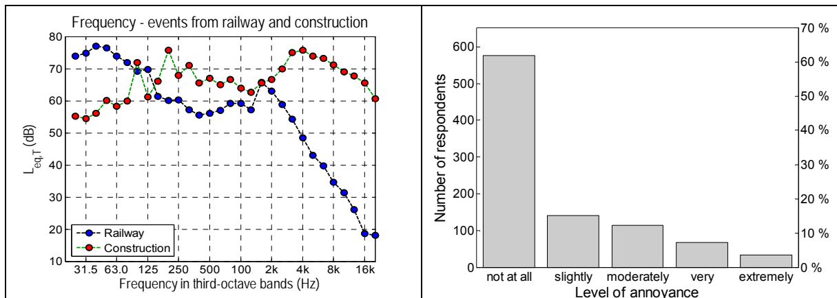
Figure 3: This figure presents, on left-hand side graph, the comparison between noise spectrum from railway and construction. The right-hand side graph presents number of respondents exposed to railway noise versus level of annoyance in 5-point semantic scale (DD ISO/TS 15666:2003).
