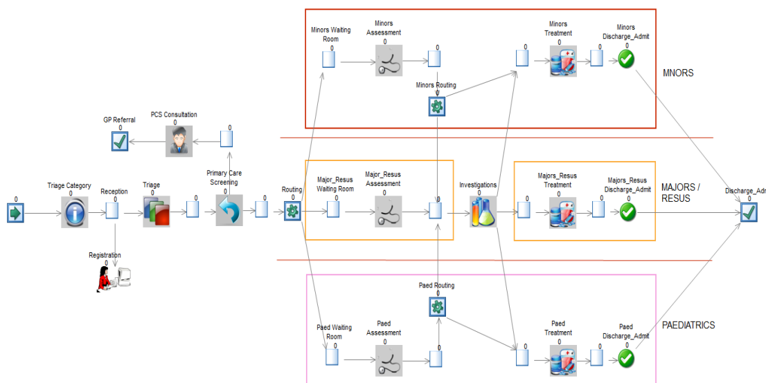
Figure 3 – Screen print of the DES model
