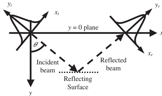
Figure 3. Sketch of a Gaussian shaped beam totally reflecting from a surface.
