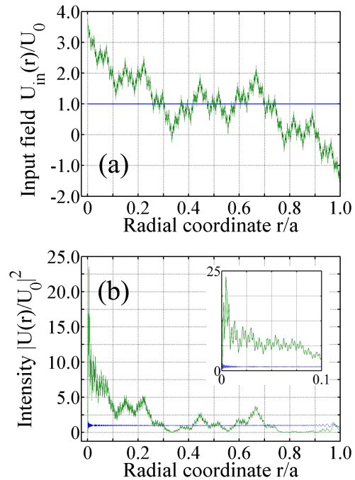
Figure 1: (a) Illumination across a circular aperture corresponding to a plane wave (blue) and a Weierstrass function with fractal dimension D_0 = 1.6 and \gamma = 3 (green). (b) Diffracted intensity patterns when N_F = 1000 .
