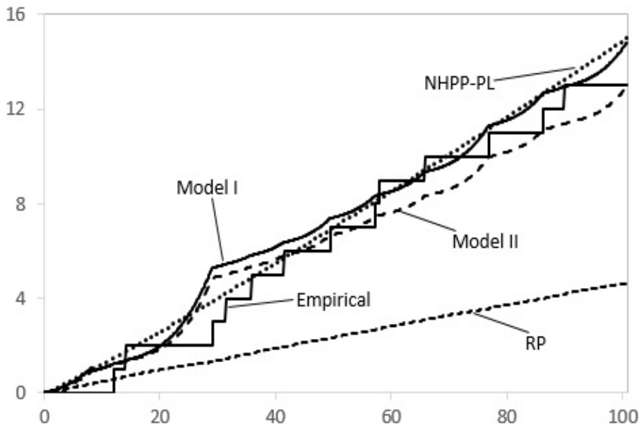
Fig. 5. The cumulative number of failures (“empirical”) and the CDFs for the models fitted to the simulated times between failures given in Table 6.
