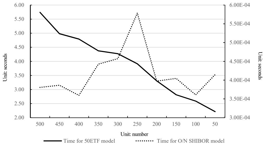
Figure 1. Average Time Required for a Single Sample of Parameters under MCMC-LV
