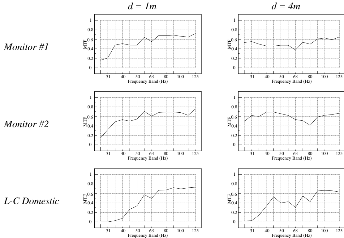
Figure 3 MTFs of 3 Loudspeakers in a Very Reverberant Live Room at Different Distances d from the Loudspeakers
