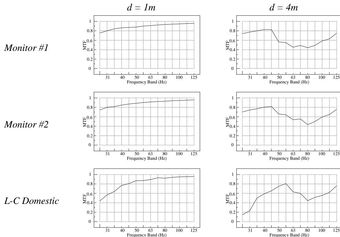
Figure 6 MTFs of 3 Loudspeakers in a Very Reverberant Live Room at Different Distances d from the Loudspeakers after Equalisation
