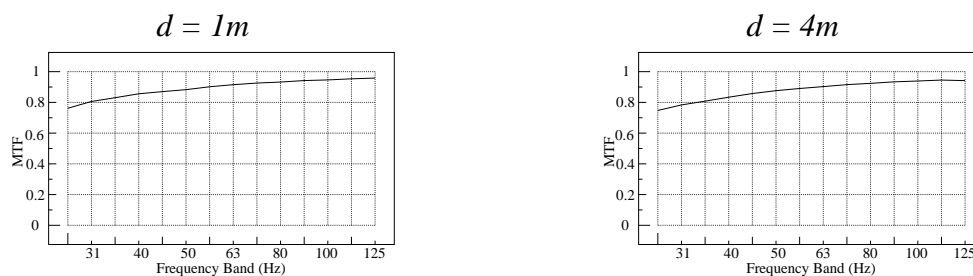
Figure 4 MTFs of a Wide Range Monitor System in a Very Highly Damped Studio Control Room at Different Distances d from the Loudspeaker after Equalisation
