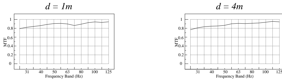
Figure 1 MTFs of a Wide Range Monitor System in a Very Highly Damped Studio Control Room at Different Distances d from the Loudspeaker
