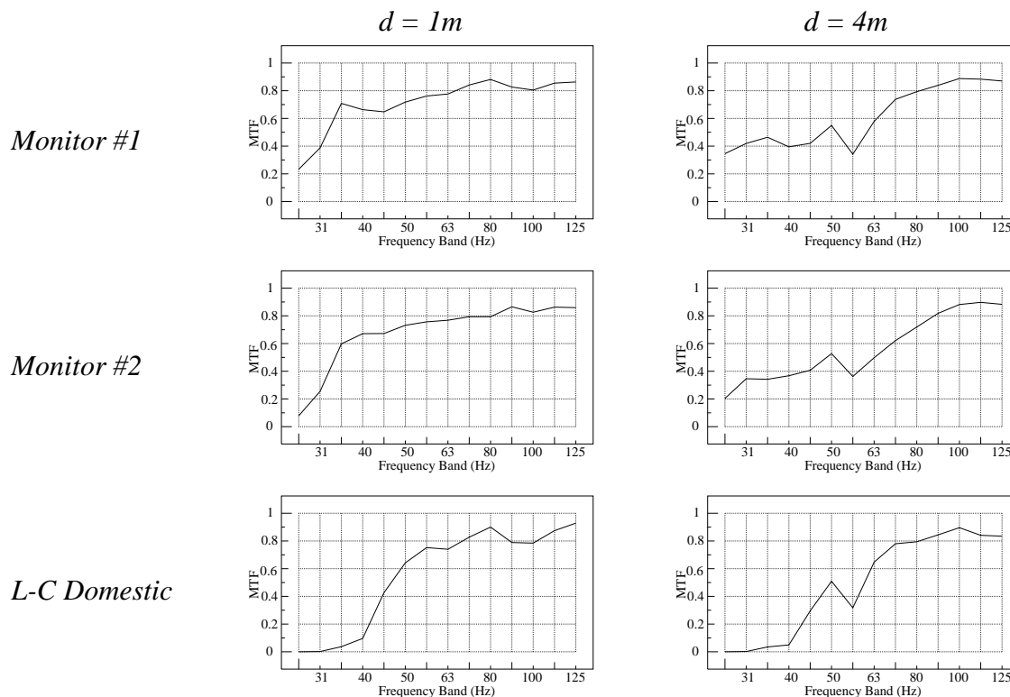
Figure 2 MTFs of 3 Loudspeakers in a Reasonably Well Damped Studio Recording Room at Different Distances d from the Loudspeakers
