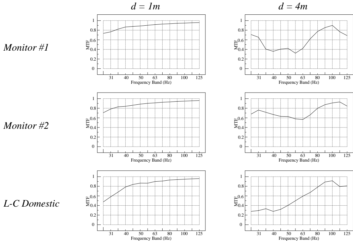
Figure 5 MTFs of 3 Loudspeakers in a Reasonably Well Damped Studio Recording Room at Different Distances d from the Loudspeakers after Equalisation
