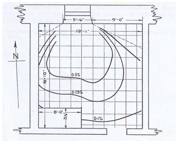
Figure 2: Pre-prepared room plan from the 1931 report on daylight in government offices which confirmed the validity of the 0.2 per cent “grumble point”. The contours representing the sky factors for 0.5 per cent, 0.25 per cent and 0.1 per cent were plotted in advance of the investigations.
