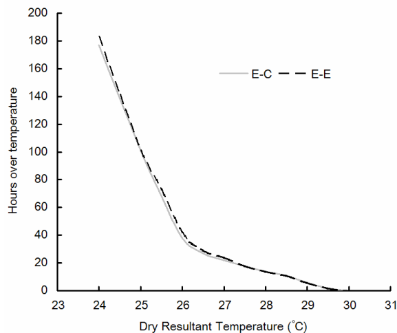
Figure 12 Number of hours over certain temperatures for the edge-in strategies.
