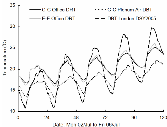
Figure 13 Office DRTs for both C-C and E-E strategies illustrating the effects of plenum.
