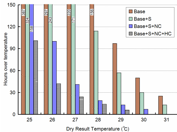
Figure 7 Number of hours over certain internal dry-resultant temperatures for all four cases.
