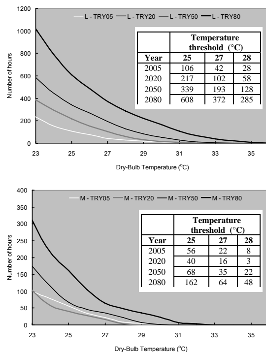
Figure 3 Total hours above stated ambient dry-bulb temperature in a current typical year, the CIBSE 2005 TRY, and in typical future years 2020, 2050 and 2080 TRYs: (a) London and (b) Manchester
