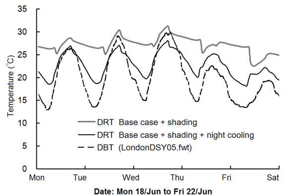
Figure 5 Comparison of resultant temperatures (DRT) for Case 3 with -, and Case 2 without, night cooling.
