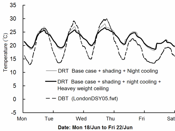
Figure 6 Comparison of dry resultant temperatures (DRT) for Case 3 with a light weight ceiling and Case 4 with a heavy weight ceiling.
