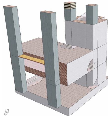
Figure 2 axonometric view of the model showing C-C ANV strategy
