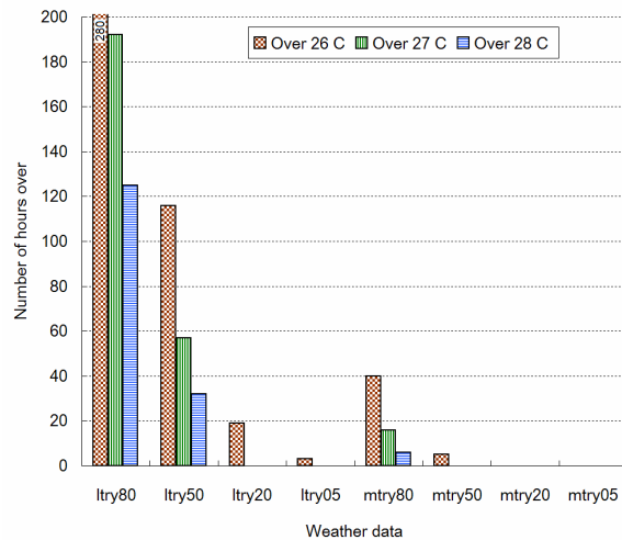
Figure 11 Predicted number of hours for which the internal DRT exceeds various values: current and future TRYs for London and Manchester
