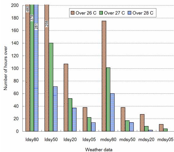
Figure 10 Predicted number of hours for which the internal DRT exceeds various values: current and future DSYs for London and Manchester
