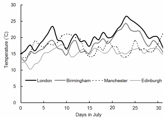
Figure 8 Daily mean external dry-bulb temperatures in July for London, Birmingham, Manchester and Edinburgh (DSYs 2005)
