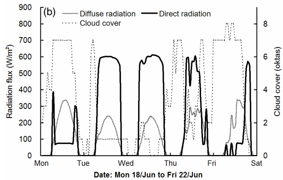
Figure 4 Internal heat gain, solar gains for the base case and the base case with 1.0m overhang shading (a) and the external solar radiation and cloud cover conditions (b).
