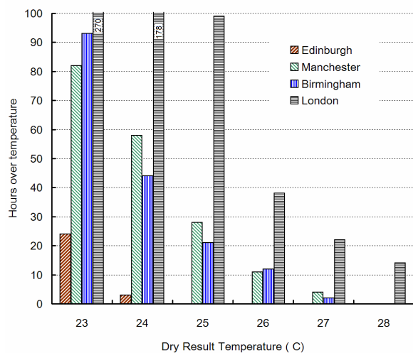
Figure 9 Predicted number of hours for which the internal DRT, when using E-E strategy, will exceed certain values at four locations in the UK: current (DSY 2005) weather data
