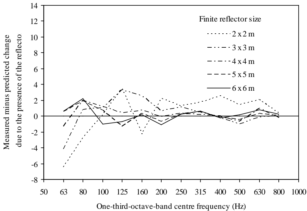
Fig. 9 Difference between the measured (finite reflector) and predicted (semi-infinite reflector) change in sound pressure level due to the presence of the reflector.
