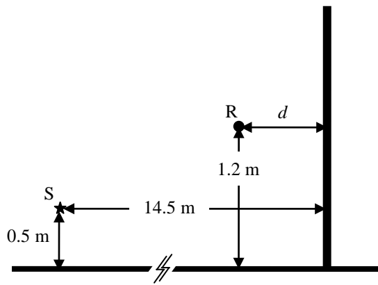
Fig. 1 Source-receiver-reflector geometry used for the comparison of measured and predicted data. These dimensions correspond to the full-scale situation for a real facade although a 1:5 scale model was used for the measurements.
