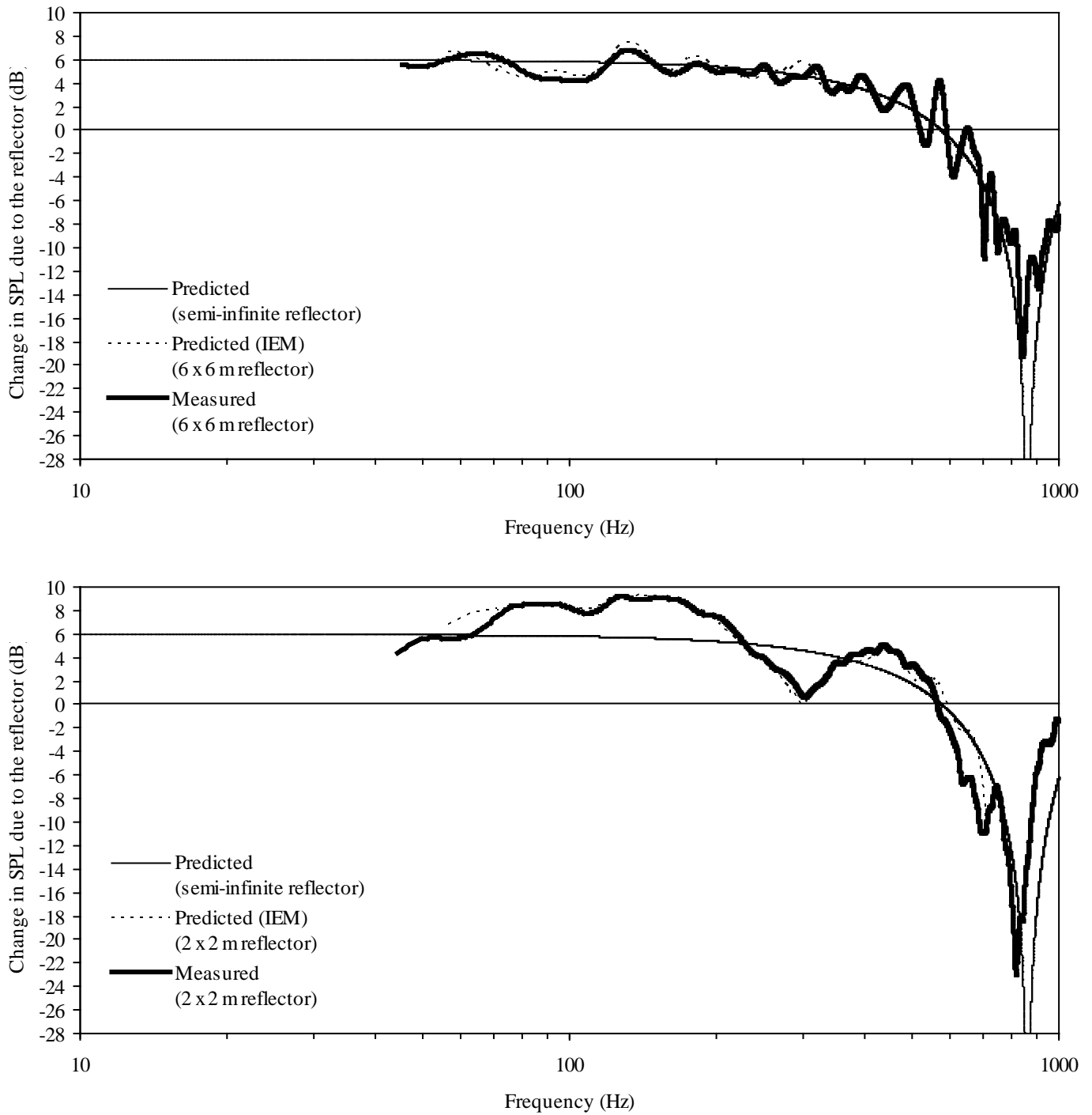
Fig. 5 Change in the sound pressure level due to the presence of the reflector: receiver-reflector distance, d=0.1 m.
