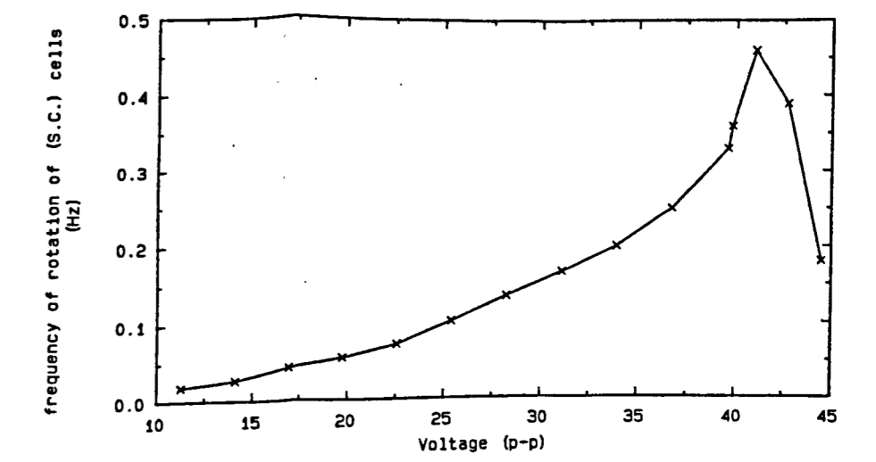
GRAPH (8.7), Signal frequency 30 KHz.
