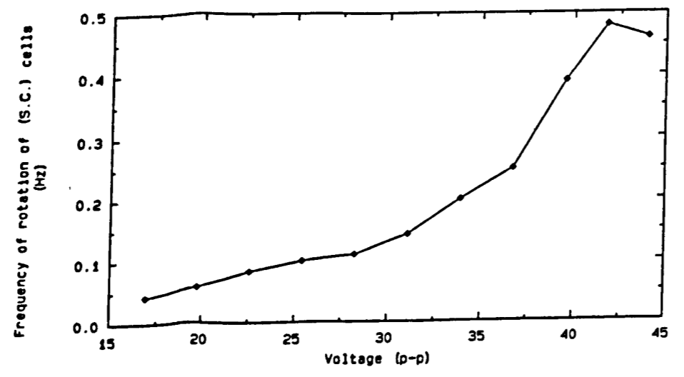
GRAPH (8.9), Signal frequency 50 KHz.
