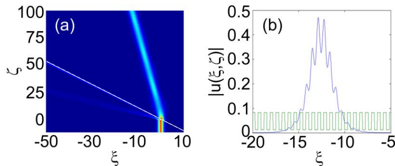
Fig. 3. Simulation showing side-coupling of an oblique spatial soliton beam (incidence angle of 10^\circ in the laboratory frame) into a coupled waveguide array (c.f. Fig. 2). (a) Numerical solution for the envelope |u(\xi, \zeta)| . (b) The field inside the array is periodic and its amplitude is modulated by a sech-type envelope.
