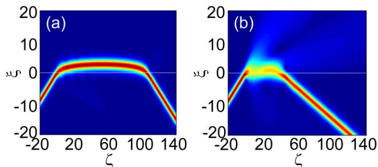
Fig. 1. (a) Simulations of typical GH shifts in the propagation plane (with normalized spatial coordinates \xi and \zeta ). These shifts are characterized by external refraction, and involve (a) linear and (b) nonlinear interfaces. The soliton interaction with the linear interface is relatively 'clean', while much more radiation is generated in the nonlinear scenario.
