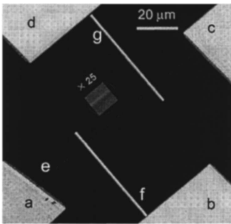
FIG. 1. A typical SEM image of an FIB-induced CVD fabricated W-Ga-C nanowire with W-Ga-C contact electrodes. The four pads are designated as a, b, c, d ; the nanowire is labeled as e (80 nm in width) and the interconnect strips as f and g for simplicity of discussion.
