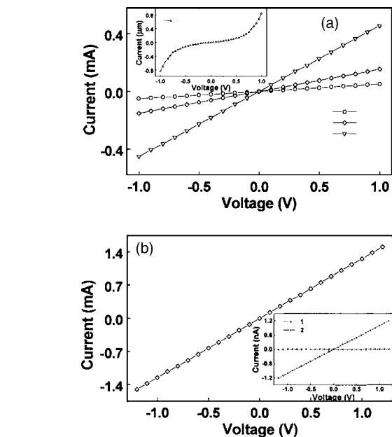
FIG. 2. (a) Room-temperature current-voltage characteristics of contact pads and interconnect strips (length: 80 μm, width: 0.63 μm) deposited with different ion doses (ions/cm 2 ): 5.8 \times 10^{18} (○); 1.2 \times 10^{19} (◇); 1.7 \times 10^{19} (▽). Inset (Δ) is the nonlinear I-V curve for the strip with an ion dose of 4.6 \times 10^{16} ions/cm 2 . (b) Linear I-V curve for a strip (length: 40 μm, width: 1.25 μm) formed to estimate the resistance of interconnect strip f in Fig. 1. The inset indicates the leakage currents measured by: (curve 1) probes on contact pads without bridge strips and (curve 2) probes placed directly on the substrate.
