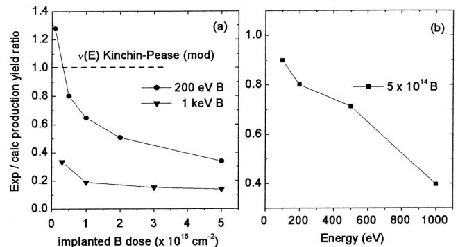
FIG. 3. (a) Experimental damage production yields in Si for 200 eV and 1 keV B^+ ions over the modified Kinchin-Pease damage production yield ratio given by Eq. (1); (b) idem as function of energy for a B^+ ion dose of 5 \times 10^{14} \text{ cm}^{-2} .
