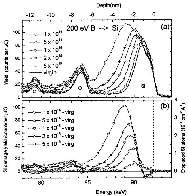
FIG. 2. MEIS spectra of (a) Si(100) before and after implantation with 200 eV B^+ ions to doses between 1 \times 10^{14} to 5 \times 10^{15} \text{ cm}^{-2} and (b) after subtraction of the virgin Si spectrum showing damage depth profiles.
