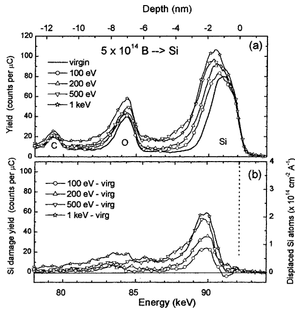
FIG. 1. MEIS spectra of (a) Si(100) before and after implantation with B^+ ions to a dose of 5 \times 10^{14} \text{ cm}^{-2} at energies from 100 eV to 1 keV, and (b) after subtraction of the virgin Si spectrum showing damage depth profiles.
