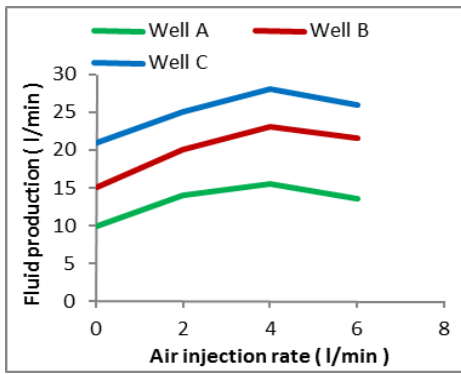
Fig. 7 Improve well performance
