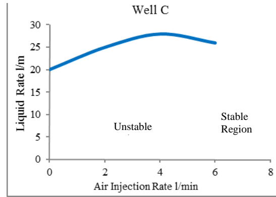
Fig. 10 Effect of injection rate on well performance
