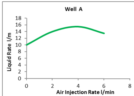
Fig. 8 The effect of injection rate on well performance at constant flow rate 10 L/min
