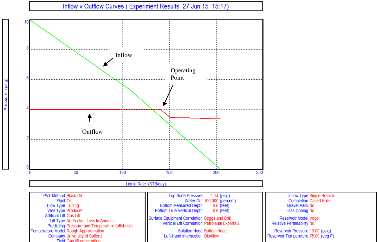
Fig. 6 Inflow and out flow relationship
