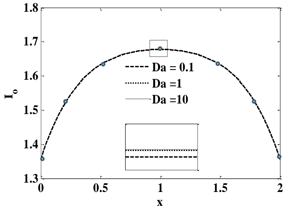
Fig. 10: Dimensionless zero moment of intensity ( I_0 ) versus axial coordinate ( X ) at R = 1 , for Pr = 2.0 , Ra = 10 , Fs = 1 , \lambda = 1 , \chi = 1 , \tau_0 = 0.1 , \Theta_f = 0.5 , N = 1 , A = 2 , r_i = 0.5 for various Darcy numbers. [RAD-SPICE validation for Da = 1 ]
