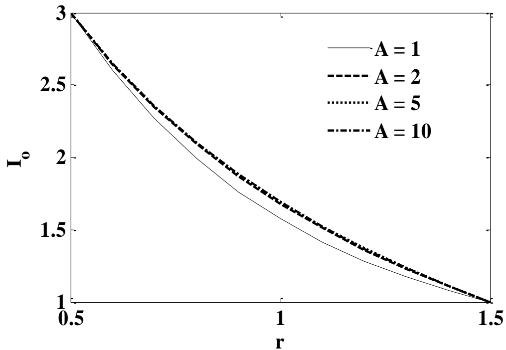
Fig. 19: Dimensionless zero moment of intensity ( I_0 ) versus radial coordinate at X = 1 , with Pr = 2.0 , Ra = 10 , Da = 0.1 , Fs = 1 , \lambda = 1 , \chi = 1 , \tau_0 = 0.1 , \Theta_f = 0.5 , N = 1 , r_i = 0.5 for various aspect ratios.
