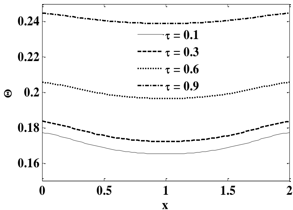
Fig. 22: Temperature ( \Theta ) versus axial coordinate ( X ) at R = 1 , with Pr = 2.0 , Ra = 10 , Da = 0.1 , Fs = 1 , \lambda = 1 , \chi = 1 , \Theta_f = 0.5 , N = 1 , r_i = 0.5 , A = 2 for various optical thickness ( \tau ) values.
