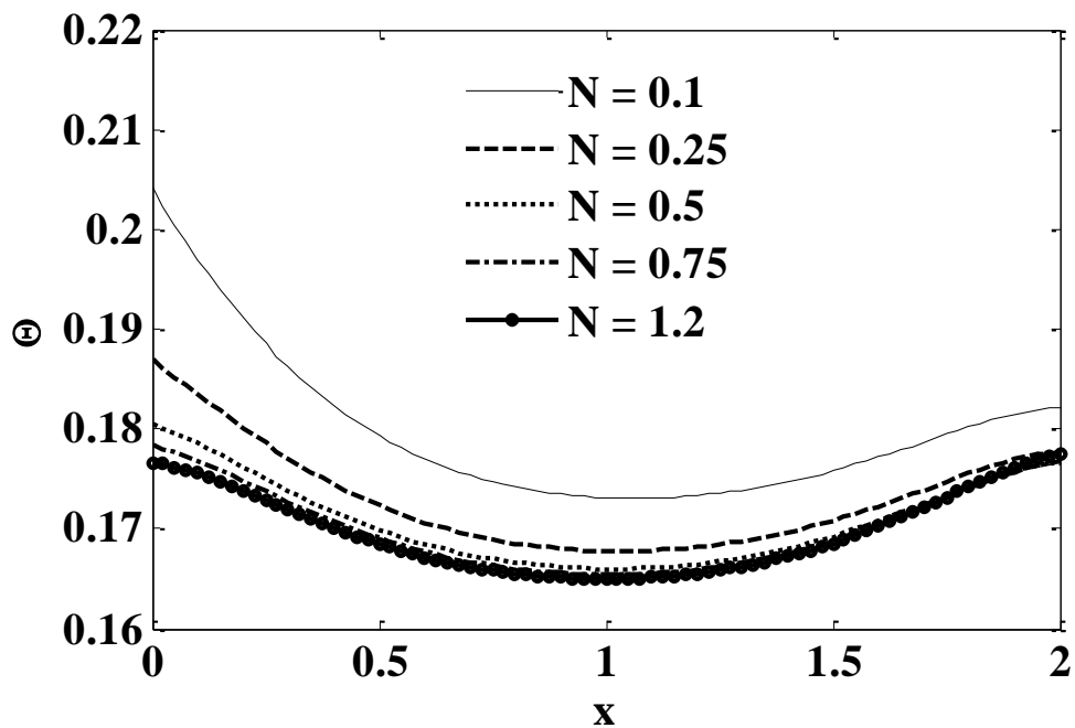
Fig. 15: Temperature ( \Theta ) versus axial coordinate ( X ) at R = 1 with Pr = 2.0 , Ra = 10 , Da = 0.1 , Fs = 1 , \lambda = 1 , \chi = 1 , \tau_0 = 0.1 , \Theta_f = 0.5 , A = 2 , r_i = 0.5 for various conduction-radiation parameters.
