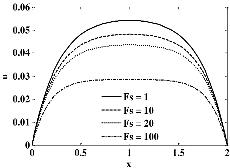
Fig. 12: Axial velocity ( U ) versus X (at R = 1 ) with Pr = 2.0 , Ra = 10 , Da = 0.1 , \lambda = 1 , \chi = 1 , \tau_0 = 0.1 , \Theta_f = 0.5 , N = 1 , A = 2 , r_i = 0.5 for various Forchheimer numbers.
