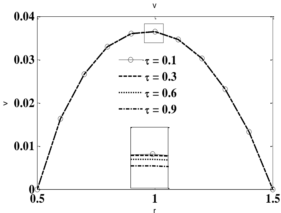
Fig. 21: Radial velocity ( V ) versus radial coordinate at X = 1 , with Pr = 2.0 , Ra = 10 , Da = 0.1 , Fs = 1 , \lambda = 1 , \chi = 1 , \Theta_f = 0.5 , N = 1 , r_i = 0.5 , A = 2 for various optical thickness ( \tau ) values.
