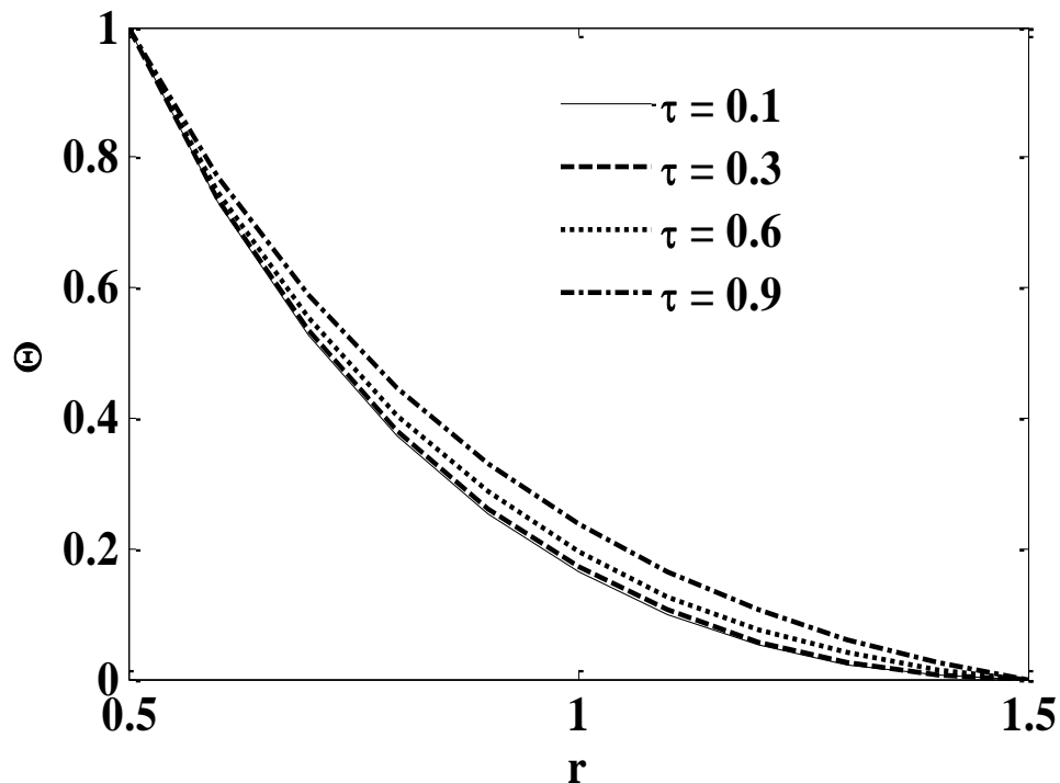
Fig. 23: Temperature ( \Theta ) versus radial coordinate at X = 1 , with Pr = 2.0 , Ra = 10 , Da = 0.1 , Fs = 1 , \lambda = 1 , \chi = 1 , \Theta_f = 0.5 , N = 1 , r_i = 0.5 , A = 2 for various optical thickness ( \tau_0 ) values.
