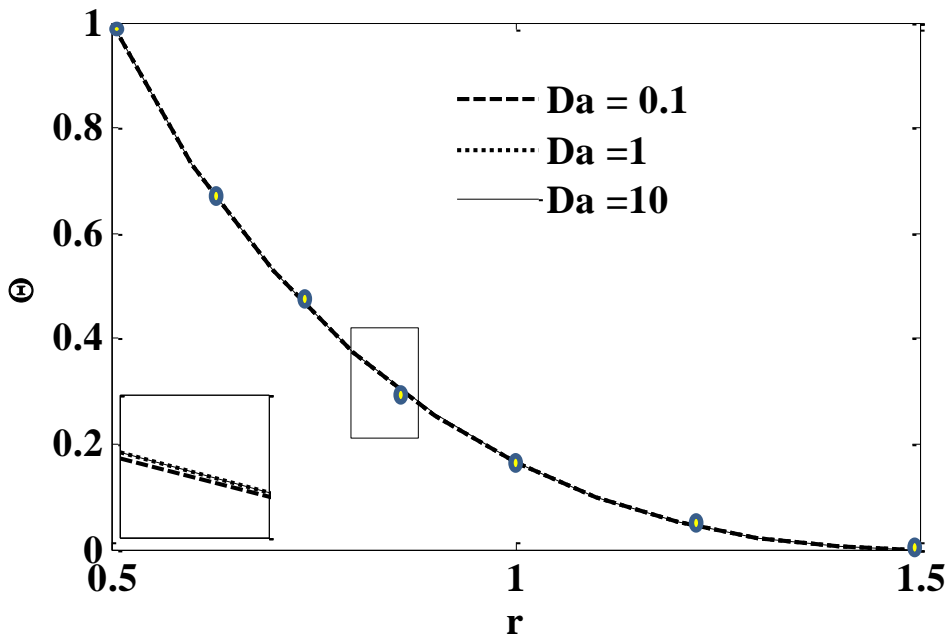
Fig. 9: Temperature ( \Theta ) versus radial coordinate at X = 1 , for Pr = 2.0 , Ra = 10 , Fs = 1 , \lambda = 1 , \chi = 1 , \tau_0 = 0.1 , \Theta_f = 0.5 , N = 1 , A = 2 , r_i = 0.5 for various Darcy numbers. [RAD-SPICE validation for Da = 1 ]
