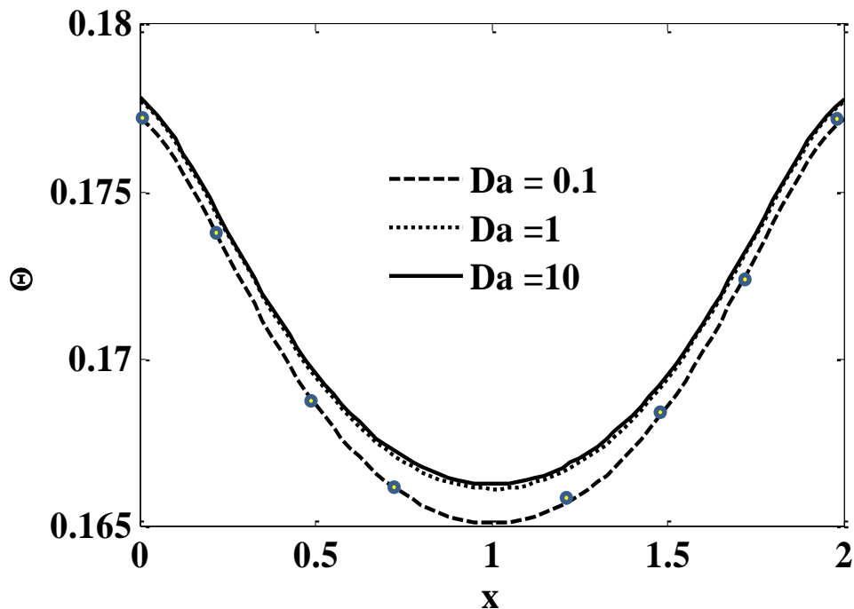
Fig. 8: Temperature ( \Theta ) versus axial coordinate ( X ) at R = 1 , for Pr = 2.0 , Ra = 10 , Fs = 1 , \lambda = 1 , \chi = 1 , \tau_0 = 0.1 , \Theta_f = 0.5 , N = 1 , A = 2 , r_i = 0.5 for various Darcy numbers. [RAD-SPICE validation for Da = 0.1 ]
