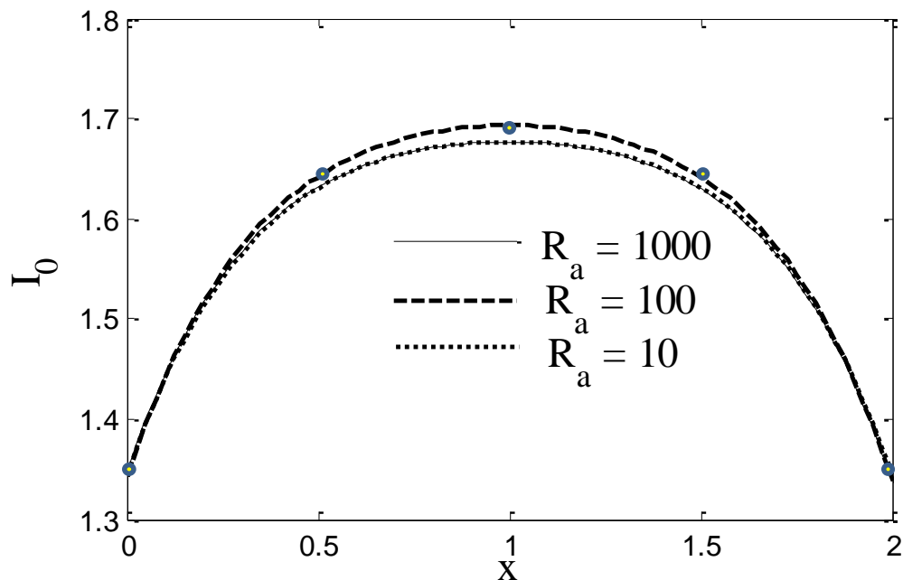
Fig 5: Dimensionless zero moment of intensity ( I_0 ) versus X (at R = 1 ) for Pr = 2.0 , Da = 0.1 , Fs = 1 , \lambda = 1 , \chi = 1 , \tau_0 = 0.1 , \Theta_f = 0.5 , N = 1 , A = 2 , r_i = 0.5 for various Rayleigh numbers. [RAD-SPICE case validated for R_a = 100 ]
