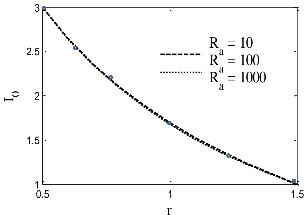
Fig. 6: Dimensionless zero moment of intensity ( I_0 ) versus radial coordinate (at X = 1 ) for Pr = 2.0 (water), Da = 0.1 (high permeability), Fs = 1 (weak quadratic porous drag), \lambda = 1 , \chi = 1 , \tau_0 = 0.1 , \Theta_f = 0.5 , N = 1 , A = 2 , r_i = 0.5 for various Rayleigh numbers. [RAD-SPICE validation for R_a = 10 ]
