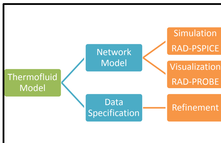
Fig. 2: RAD-PSPICE network simulation methodology
