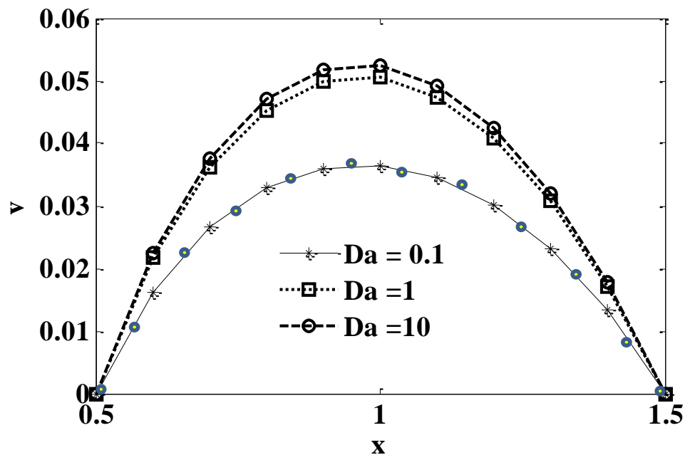
Fig. 7: Radial velocity versus X (at R = 1 ) for Pr = 2.0 , Ra = 10 , Fs = 1 , \lambda = 1 , \chi = 1 , \tau_0 = 0.1 , \Theta_f = 0.5 , N = 1 , A = 2 , r_i = 0.5 for various Darcy numbers. [RAD-SPICE validation for Da = 0.1 ]
