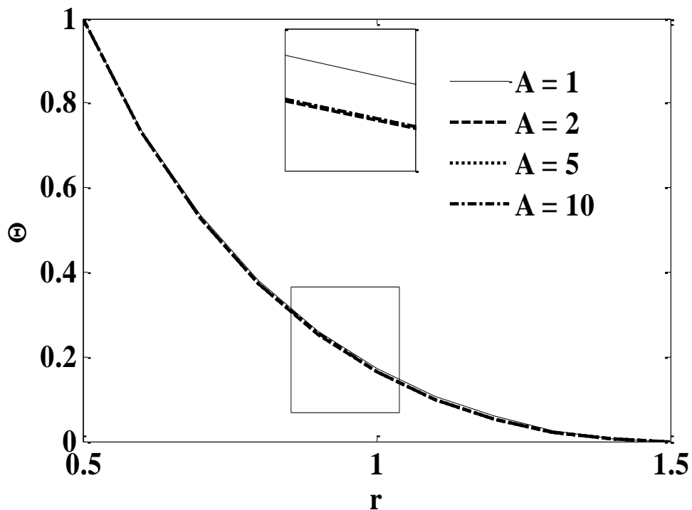
Fig. 18: Temperature ( \Theta ) versus radial coordinate, at X = 1 , with Pr = 2.0 , Ra = 10 , Da = 0.1 , Fs = 1 , \lambda = 1 , \chi = 1 , \tau_0 = 0.1 , \Theta_f = 0.5 , N = 1 , r_i = 0.5 for various A values (1, 2, 5, 10).
