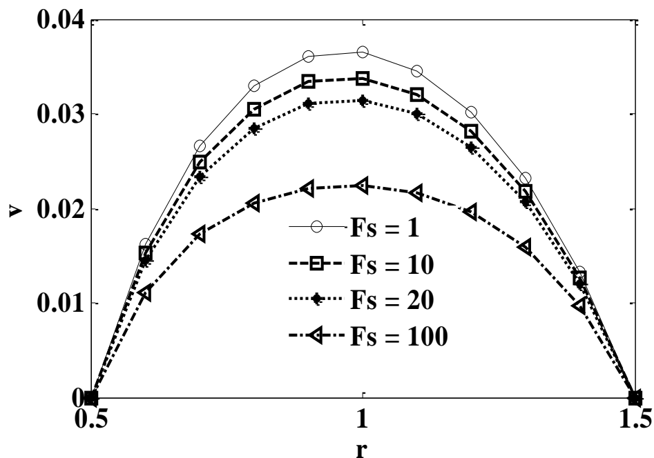
Fig. 13: Radial velocity ( V ) versus radius (at X = 1 ) with Pr = 2.0 , Ra = 10 , Da = 0.1 , \lambda = 1 , \chi = 1 , \tau_0 = 0.1 , \Theta_f = 0.5 , N = 1 , A = 2 , r_i = 0.5 for various Forchheimer numbers.
