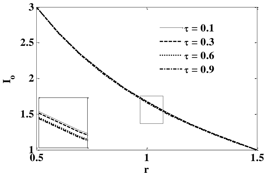
Fig. 24: Dimensionless zero moment of intensity ( I_0 ) versus radial coordinate at X = 1 , with Pr = 2.0 , Ra = 10 , Da = 0.1 , Fs = 1 , \lambda = 1 , \chi = 1 , \Theta_f = 0.5 , N = 1 , r_i = 0.5 , A = 2 for various optical thickness ( \tau_0 ) values.
