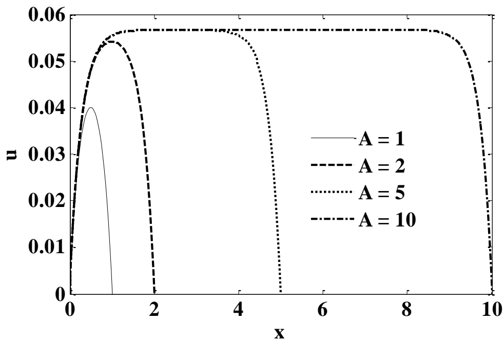
Fig. 16: Axial velocity ( U ) versus axial coordinate ( X ), at R = 1 , with Pr = 2.0 , Ra = 10 , Da = 0.1 , Fs = 1 , \lambda = 1 , \chi = 1 , \tau_0 = 0.1 , \Theta_f = 0.5 , N = 1 , r_i = 0.5 for various aspect ratio values.
