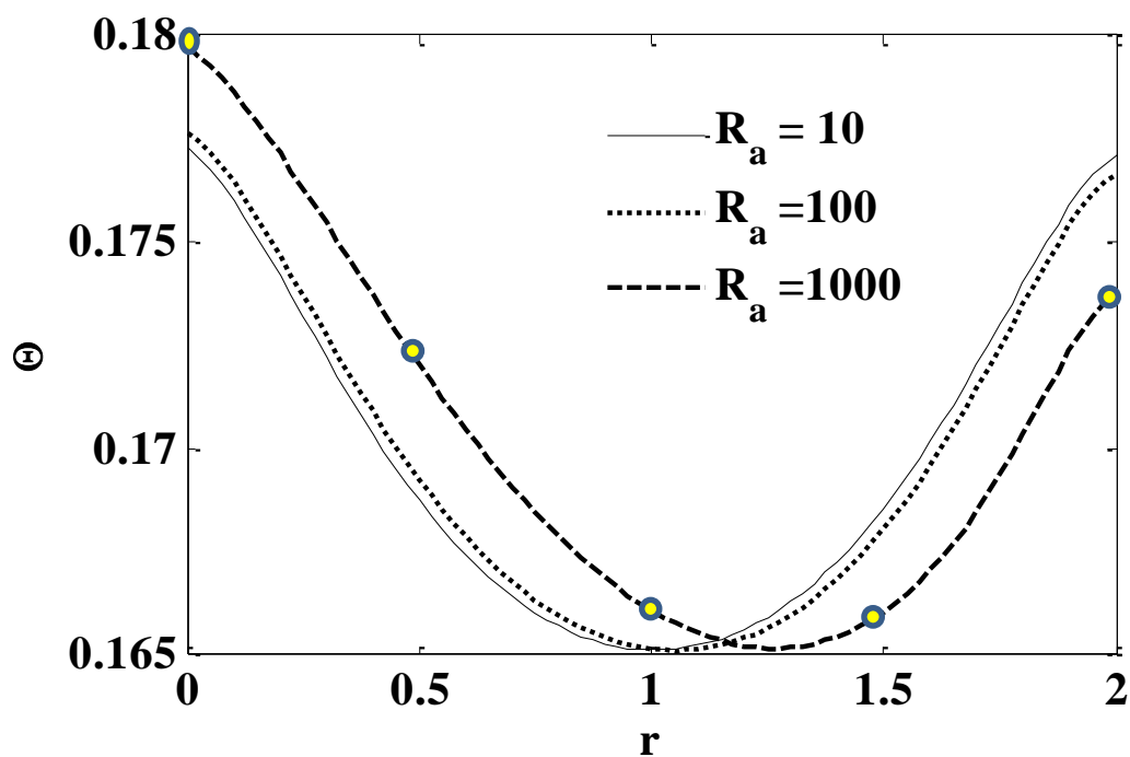
Fig 4: Temperature ( \Theta ) versus radius (at X = 1 ) for Pr = 2.0 , Da = 0.1 , Fs = 1 , \lambda = 1 , \chi = 1 , \tau_0 = 0.1 , \Theta_f = 0.5 , N = 1 , A = 2 , r_i = 0.5 for various Rayleigh numbers. [RAD-SPICE case validated for R_a = 1000 ]
