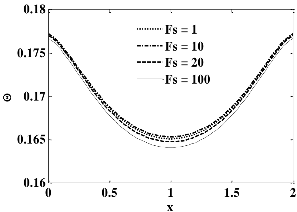
Fig. 14: Temperature ( \Theta ) versus axial coordinate, X , at R = 1 and \Theta versus R (at X = 1 ) for Pr = 2.0 , Ra = 10 , Da = 0.1 , \lambda = 1 , \chi = 1 , \tau_0 = 0.1 , \Theta_f = 0.5 , N = 1 , A = 2 , r_i = 0.5 for various Forchheimer numbers.
