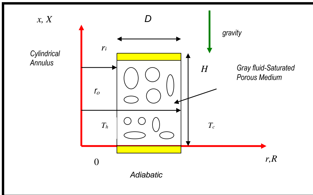
Figure 1: Radiative convection in a cylindrical isotropic porous medium annulus
