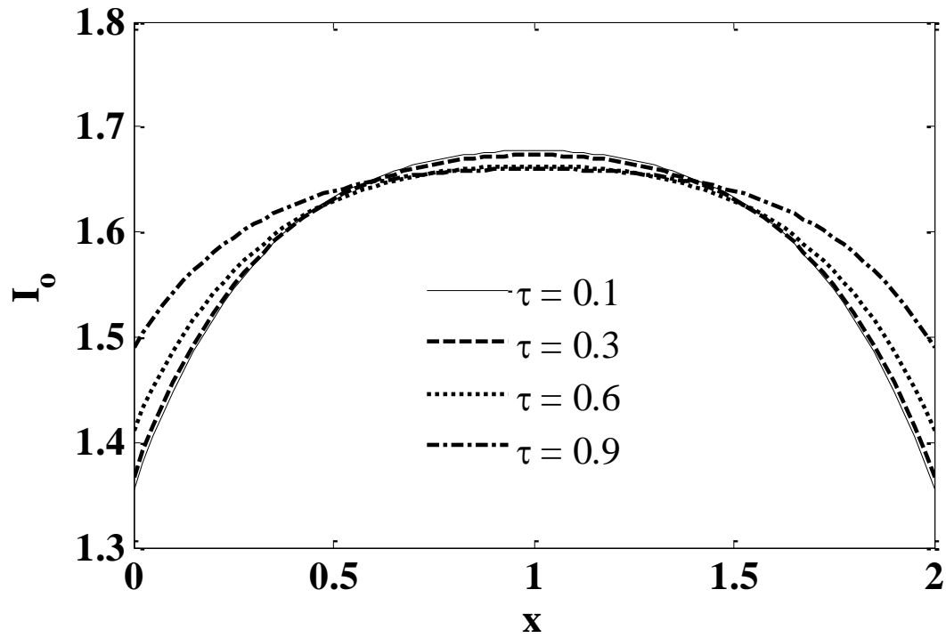
Fig. 25: Dimensionless zero moment of intensity ( I_0 ) versus axial coordinate ( X ) at R = 1 with Pr = 2.0 , Ra = 10 , Da = 0.1 , Fs = 1 , \lambda = 1 , \chi = 1 , \Theta_f = 0.5 , N = 1 , r_i = 0.5 , A = 2 for various optical thickness ( \tau ) values.
