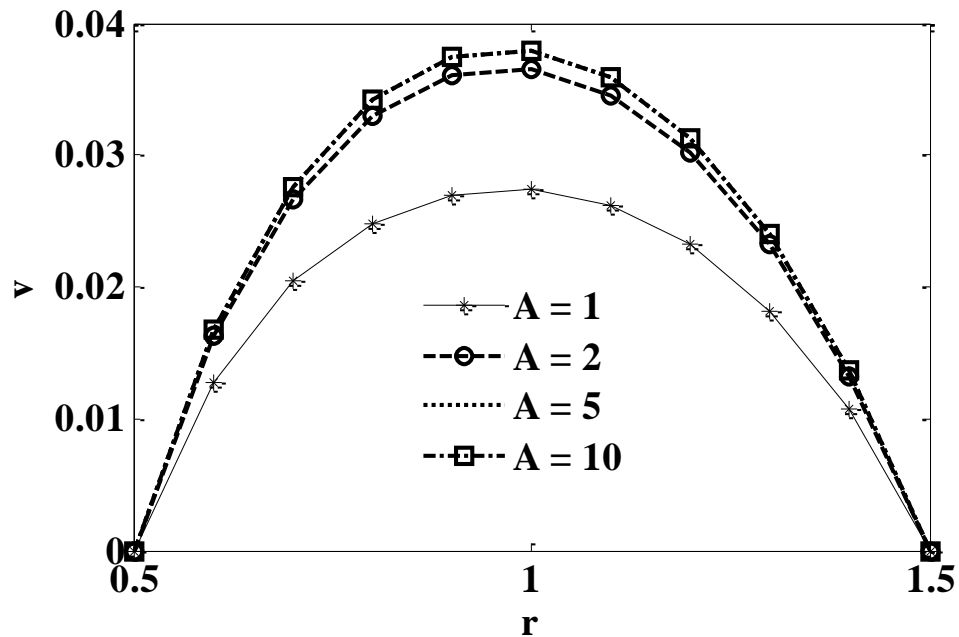
Fig. 17: Radial velocity ( V ) versus radial coordinate at X = 1 with Pr = 2.0 , Ra = 10 , Da = 0.1 , Fs = 1 , \lambda = 1 , \chi = 1 , \tau_0 = 0.1 , \Theta_f = 0.5 , N = 1 , r_i = 0.5 for various aspect ratio values.
