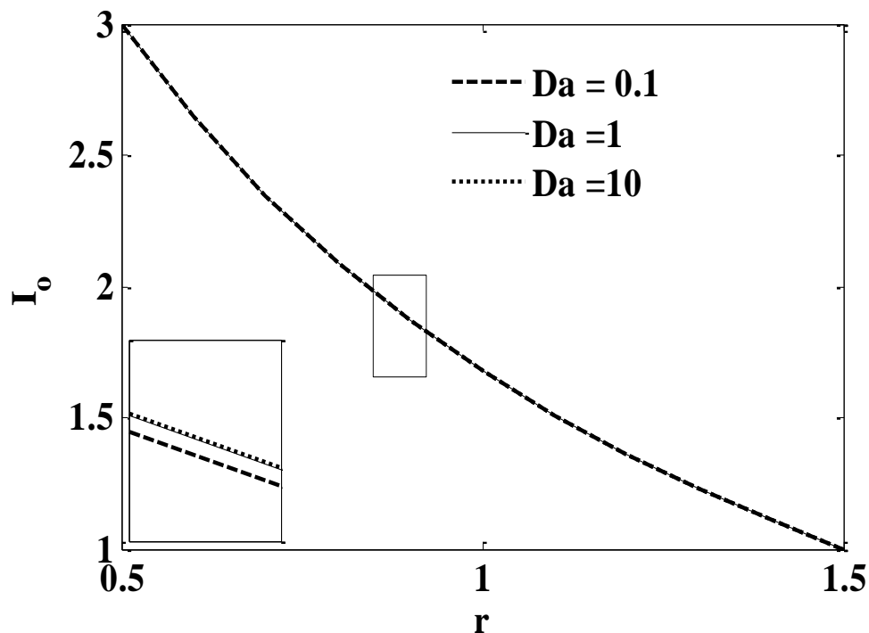
Fig. 11: Dimensionless zero moment of intensity ( I_0 ) versus radial coordinate at X = 1 , for Pr = 2.0 , Ra = 10 , Fs = 1 , \lambda = 1 , \chi = 1 , \tau_0 = 0.1 , \Theta_f = 0.5 , N = 1 , A = 2 , r_i = 0.5 for various Darcy numbers.
