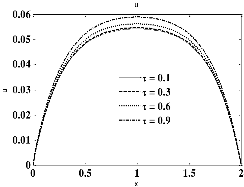
Fig. 20: Axial velocity ( U ) versus X , at R = 1 , with Pr = 2.0 , Ra = 10 , Da = 0.1 , Fs = 1 , \lambda = 1 , \chi = 1 , \Theta_f = 0.5 , N = 1 , r_i = 0.5 , A = 2 for various optical thickness ( \tau_0 ) values.
