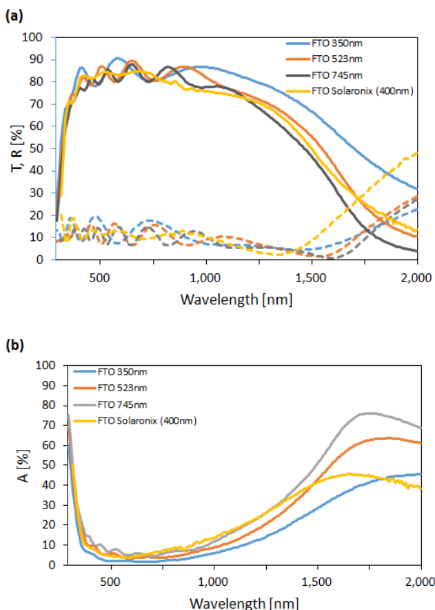
Figure 3 (a) Transmittance (solid line) and reflectance (dotted line), (b) absorbance.
