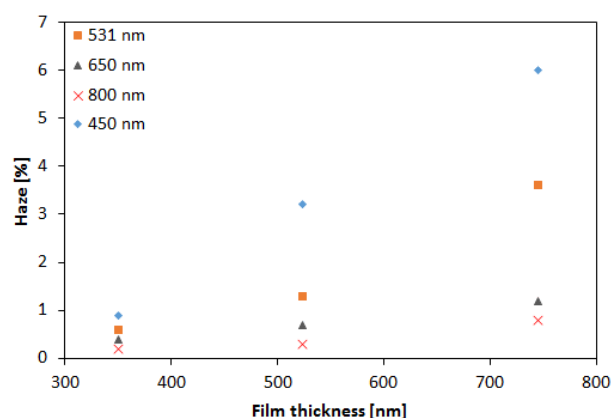
Figure 2 Optical haze for Set D at 4 different wavelengths.
