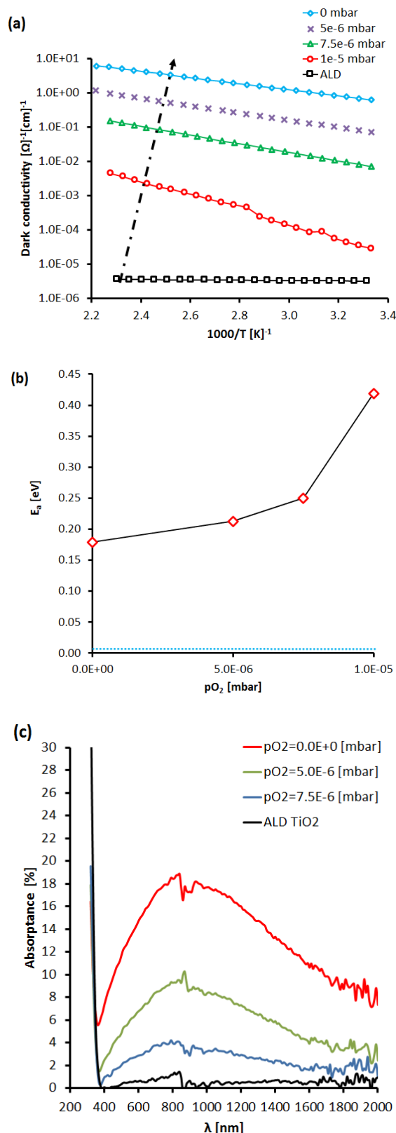
Figure 4 (a) Arrhenius plot of the surface conductivity of sputtered \text{TiO}_{2-x} and \text{TiO}_2 by ALD thin films, showing that the bulk conductivity of these thin films increases with the degree of reduction. (b) Activation energy ( E_a ) as a function of the partial \text{O}_2 pressure ( p\text{O}_2 ), the blue line corresponds to the 7meV of ALD deposited \text{TiO}_{2-x} . (c) Optical absorbance of \text{TiO}_{2-x} thin films with different p\text{O}_2 .
