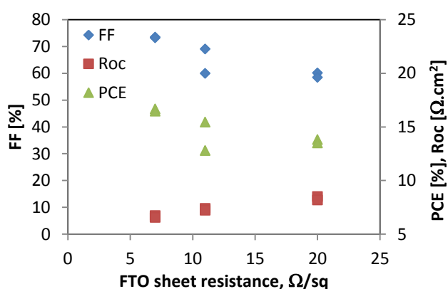
Figure 5 The trend in cell parameters for FTO Set D for the cells fabricated using the sputtered TiO 2-x layer.
