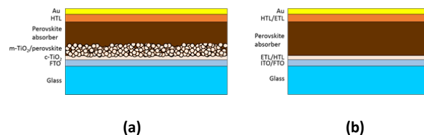
Fig. 1 Schematics of a perovskite based cell (a) mesoscopic, (b) planar.
