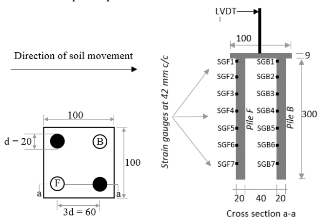
Fig. 4 Details of model piles and cap.
