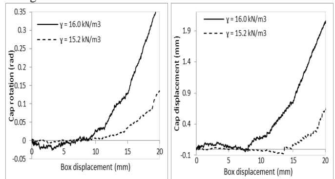
a. Rotation b. Displacement Fig. 9 Rotation and deflection of the cap versus box movement.
