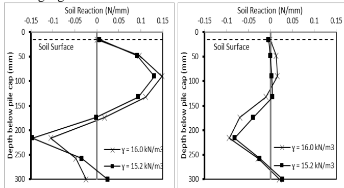
a. Pile F b. Pile B Fig. 7 Soil reaction profiles of piles at \Delta_B = 20 mm.
