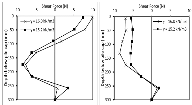
a. Pile F b. Pile B Fig. 6 Shear force profiles of piles at \Delta_B = 20 mm.
