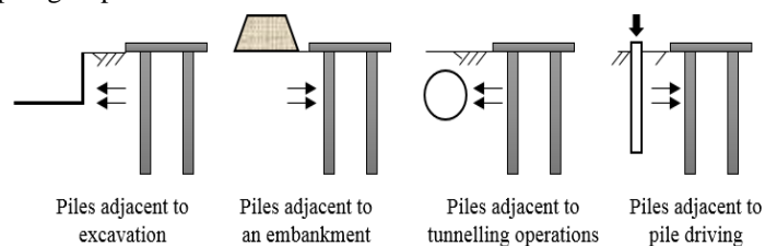
Fig. 1 Examples of passive piles.
