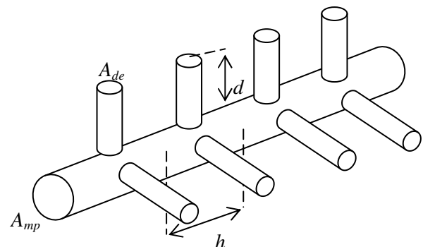
Figure 1. Main pore (cross sectional area A_{mp} ) with periodically arranged dead-end pores, N=2 identical dead-end pores with cross section A_{de} and length d per period h . The dead-ends are located at “nodes”.
