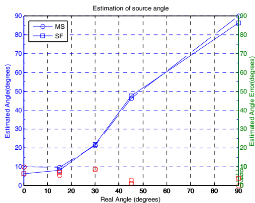
Figure 8 – Estimation of source angle from microphone signals. Comparison between mid-side (omni-fig. of 8) pair (MS) and Y/X B-Format outputs from Soundfield microphone (SF). Error for each microphone set is indicated in red. Measurements taken in a concert hall, using white noise.
