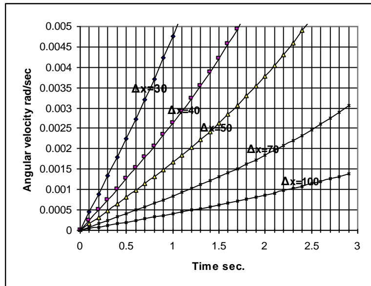
Figure 3. Relationship between angular velocity and time (assuming that leader's constant deceleration is equal to -2\text{m/sec}^2 for different initial space headways)
