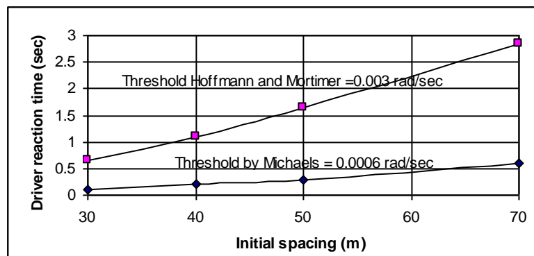
Figure 4. Relationship between driver's reaction time and initial spacing
